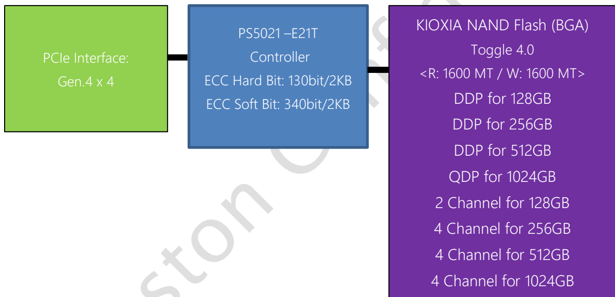
Fig 1-1: Kingston SSD OM8PGP4 Block Diagram
